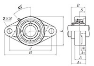
Two Bolt Rhombus Flanged Unit, Cast Housing, Set Screw, UCFL Type - Dimensions
