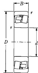
Cylindrical Bore 213
