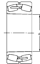
Tapered Bore 241K30 Taper 1:30
