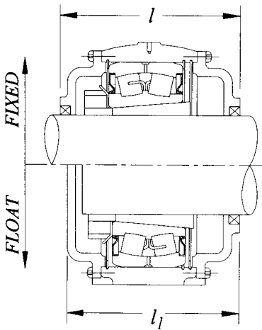
C(M)-SPW22...
