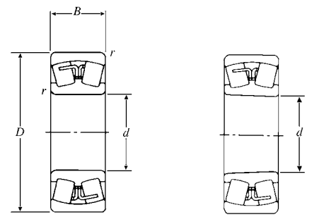
Cylindrical Bore 223B 223C Tapered Bore 223BK 223CK Taper 1:12
