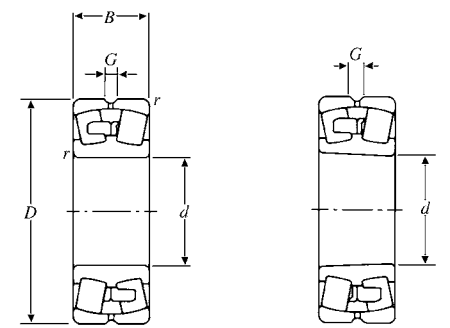
Cylindrical Bore 223B Tapered Bore 223BK Taper 1:12
