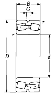
Cylindrical Bore 231
