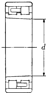
Tapered Bore NN30K Taper 1:12
