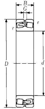
Cylindrical Bore 239
