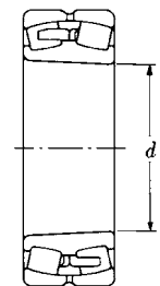
Tapered Bore 231K Taper 1:12
