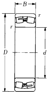
Cylindrical Bore 230
