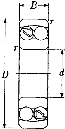
Cylindrical Bore 13
