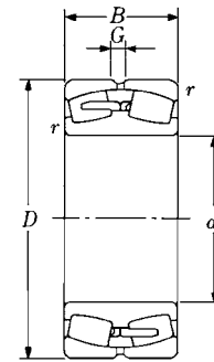
Cylindrical Bore 241
