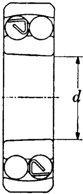
Tapered Bore 13K Taper 1:12
