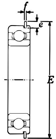
With Snap Ring TMB2NR
