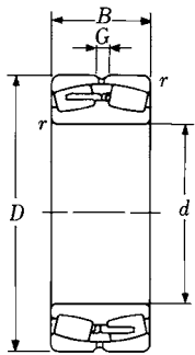
Cylindrical Bore 240
