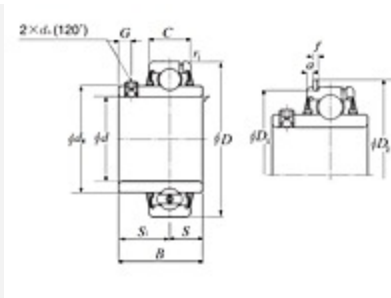
Bearing Insert w/ Set Screw, Wide Inner Ring - Cylindrical O.D., Snap Ring - Dimensions
