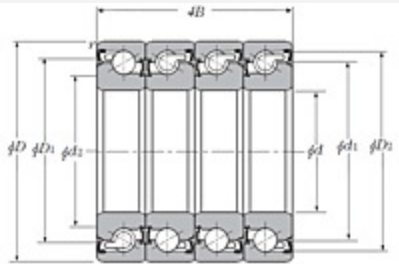
Quadruple-Row Angular Contact Thrust Ball Bearing for Ball Screws - DBTT Arrangement, Double Sealed, Three Rows Bear Axial Load - Dimensions
